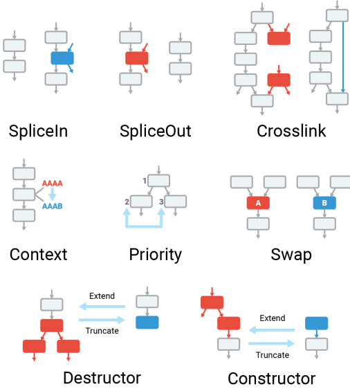
Figure 3: GraphFuzz Mutations
